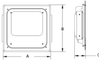
FXRC130/50K A:420mm B:420mm C:90mm
