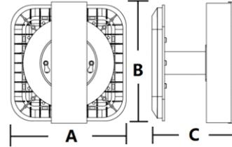
FXGSC75W : A:325mm B:325mm C:228mm FXGSC100W : A:480mm B:480mm C:245mm FXGSC150W : A:480mm B:480mm C:245mm
