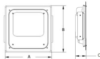
FXRC130/50K A:420mm B:420mm C:90mm
