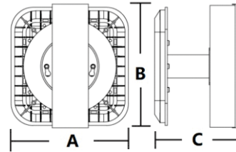
FXGSC150W/50K A:480mm B:480mm C:245mm
