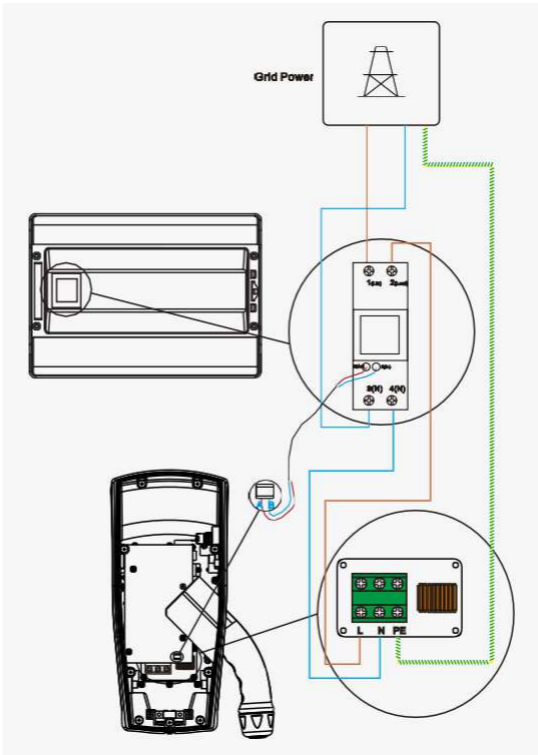
Single Phase
