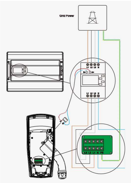
Three Phase
