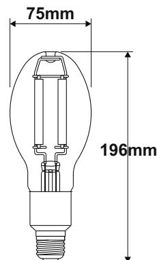
ED60/20W/E27
