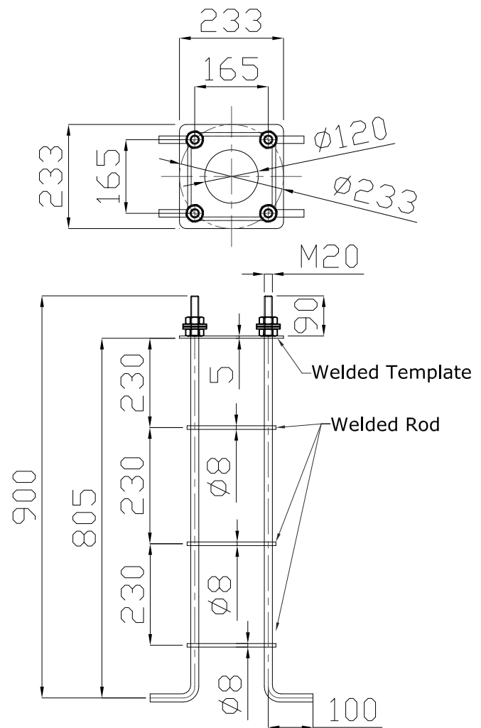
FOUNDATION CAGE M20X900
